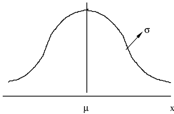
Gambar1. Kurva Distribusi Normal
